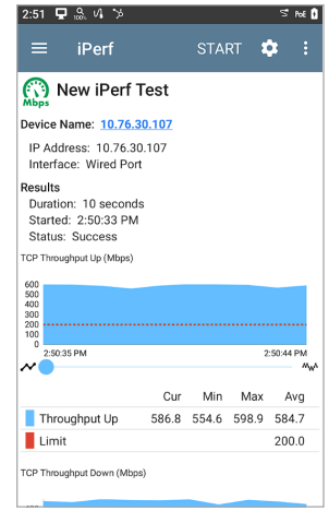
iPerf Screen
